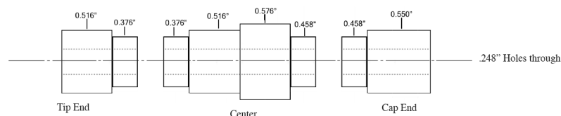
Diagram C / Bushings #PKMAJJRBU
